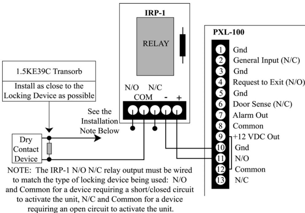
Figure 4: Adding an IRP-1 to a Dry-Contact Device - PXL-100 Configuration
