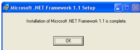
Figure 10: Installation Complete
