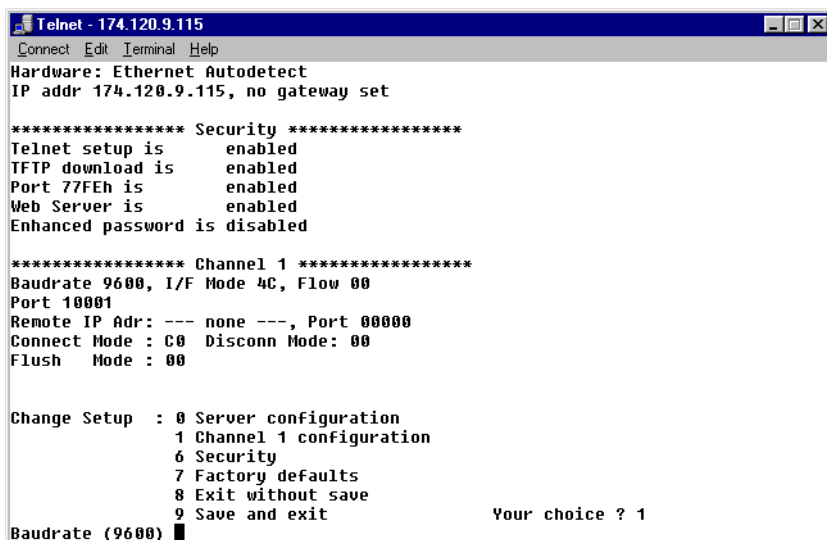
Figure 36: The First Channel 1 Configuration Parameters
