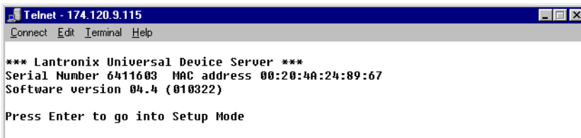
Figure 31: Enter Telnet
