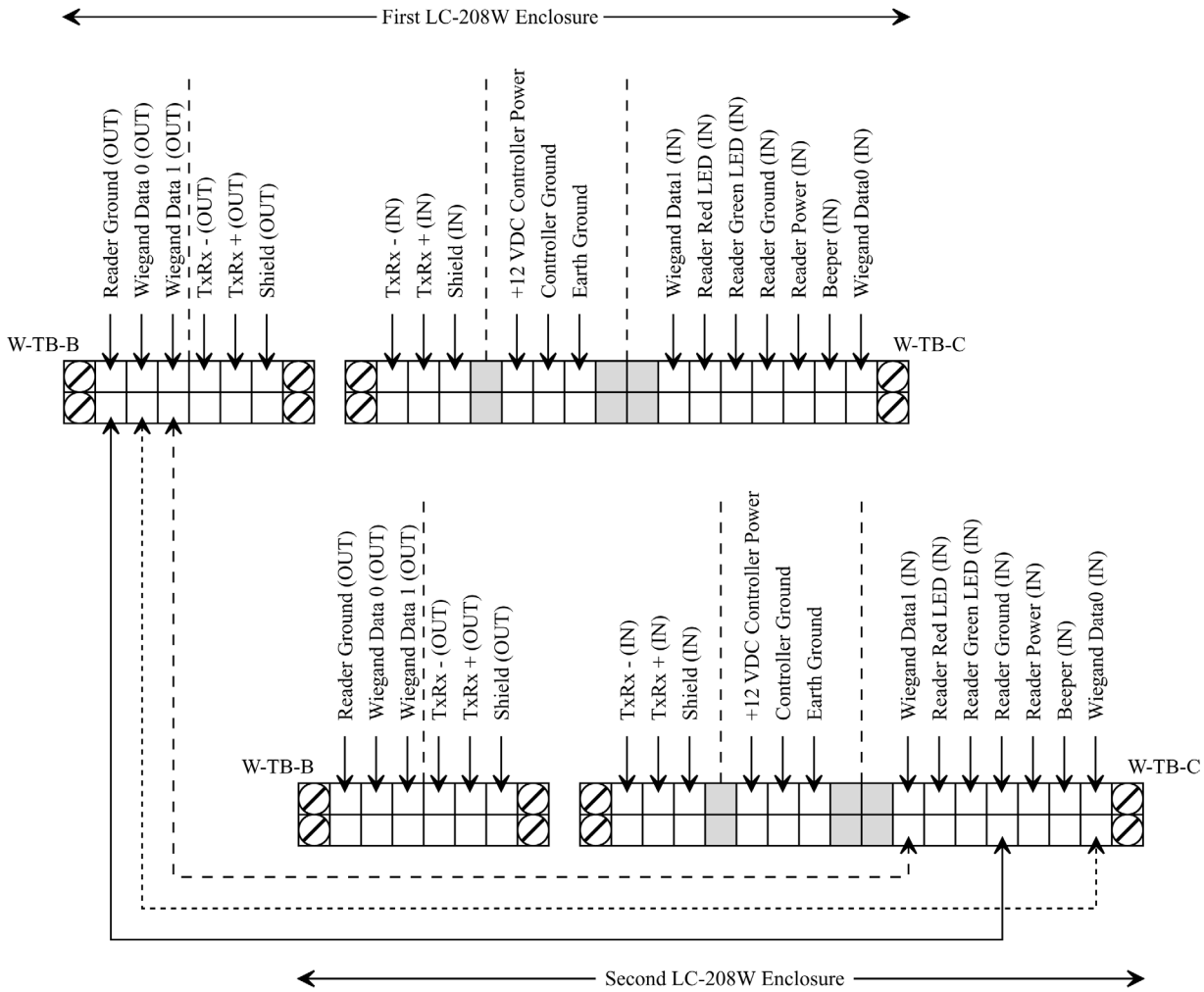
Figure 13: LC-208W to LC-208W Reader Wiring Connections
