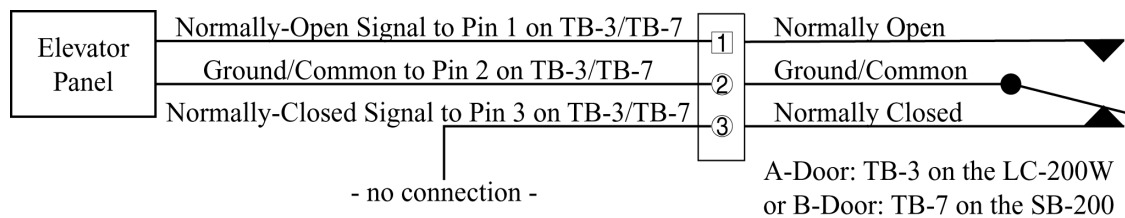
Figure 5: Floor Control Relay Connection
