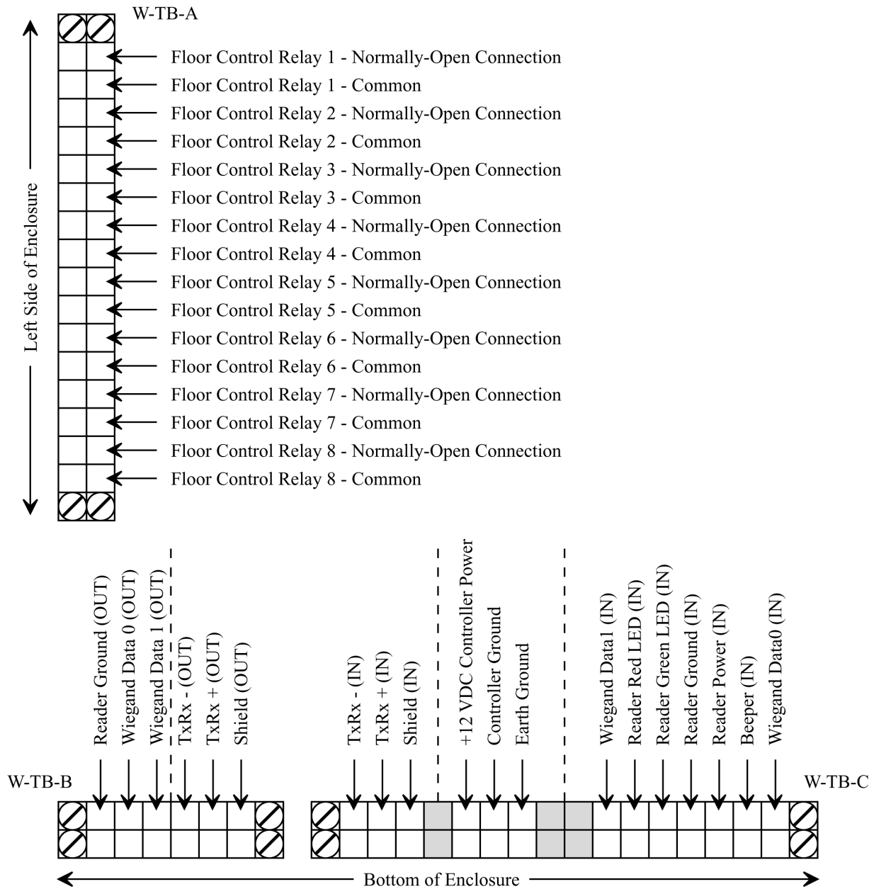
Figure 10: LC-208W Wiegand Elevator Panel Wiring Connections
