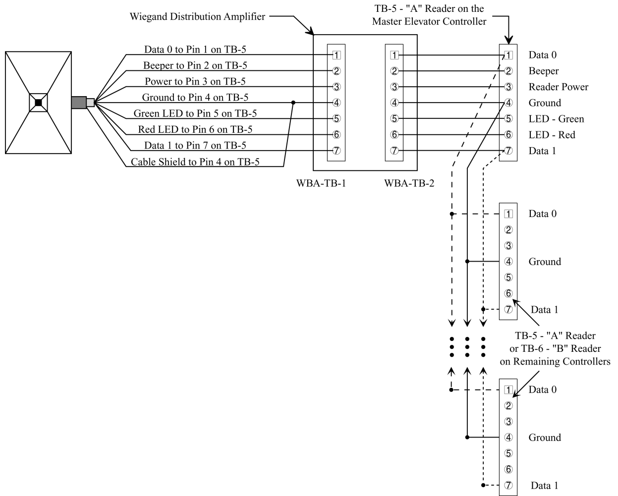
Figure 8: Daisy-Chained Wiegand Reader Connections
