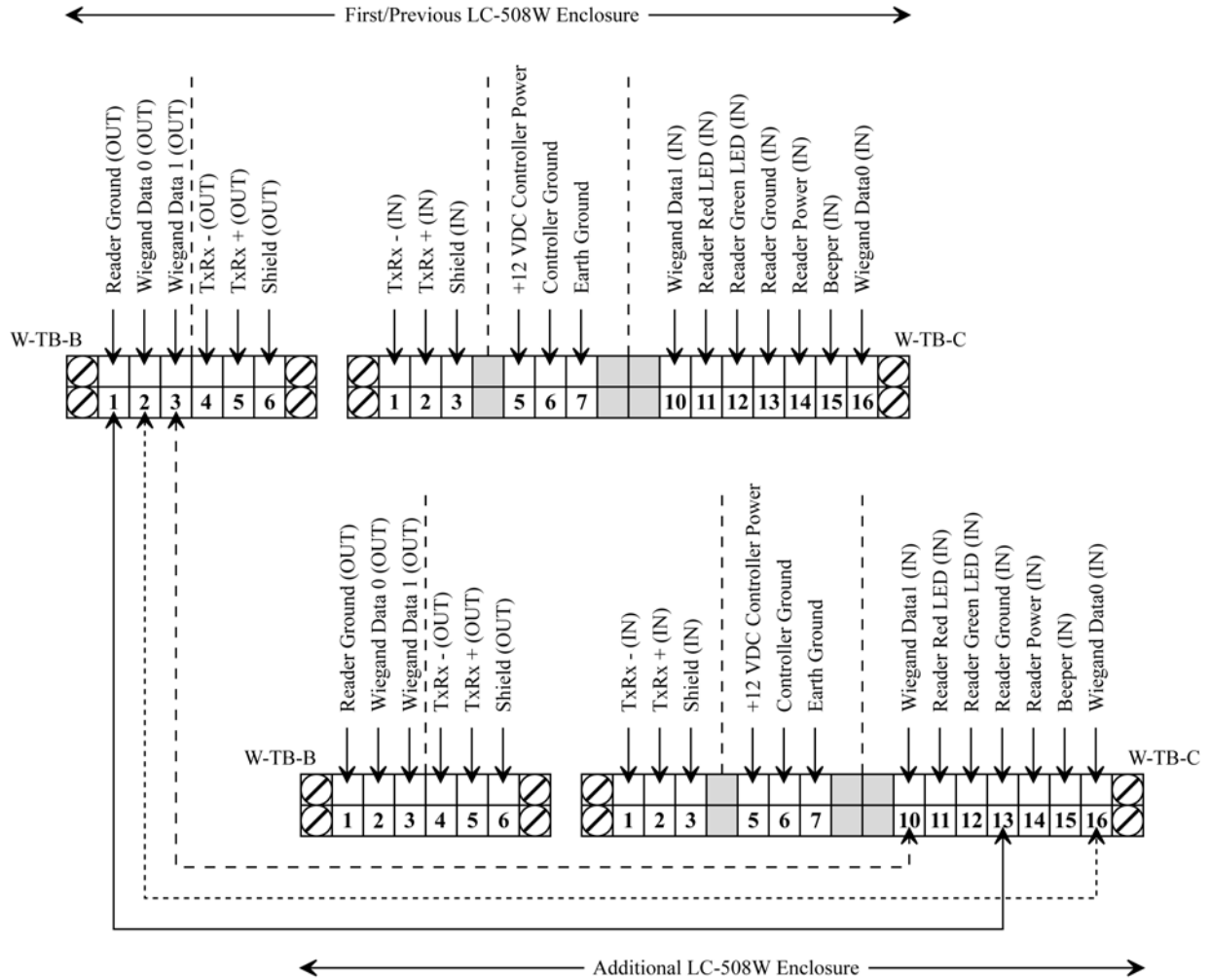
Figure 14: LC-508W to LC-508W Reader Wiring Connections
