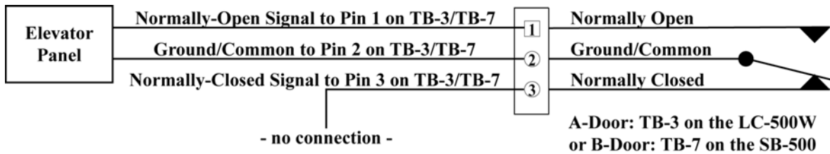
Figure 6: Floor Control Relay Connection
