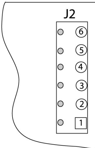
Figure 5: PXL-100/OB-7 Connections
