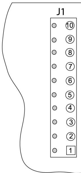
Figure 4: PXL-100/J1 Connections on the OB-7
