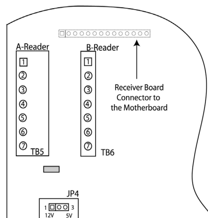
Figure 3: PXL-250W Connections
