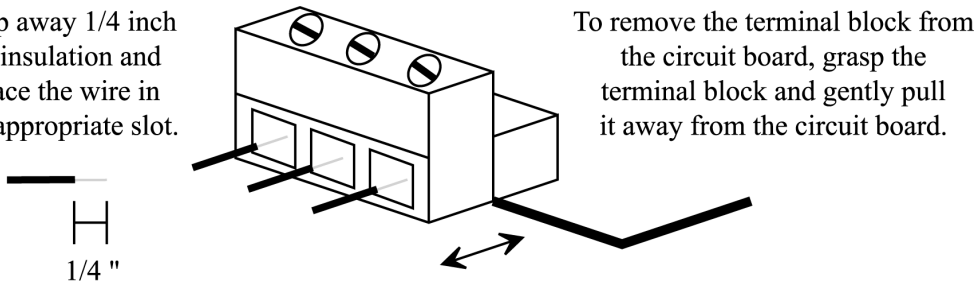
Figure 3: Connecting Wires to Terminal Blocks
