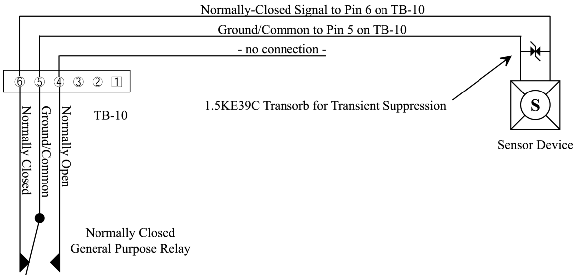
Figure 17: General Purpose Output – Normally Closed Relay
