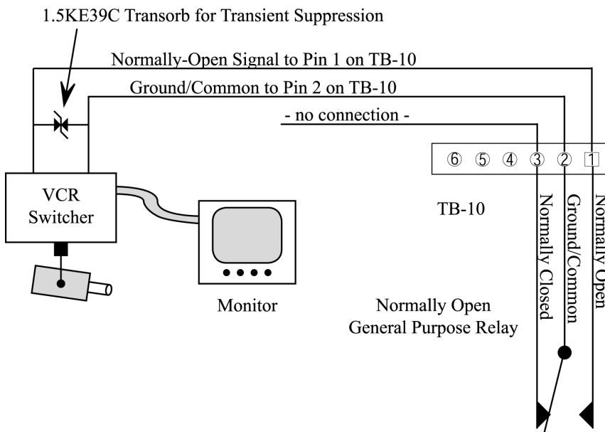
Figure 18: General Purpose Output – Normally Open Relay
