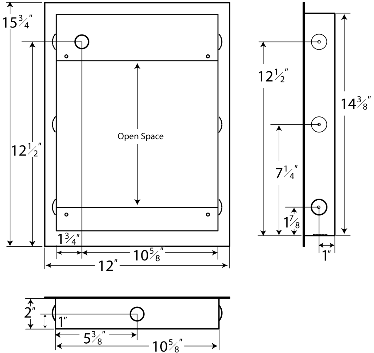
Figure 1: FMK-95 Recess Mount Dimensions
