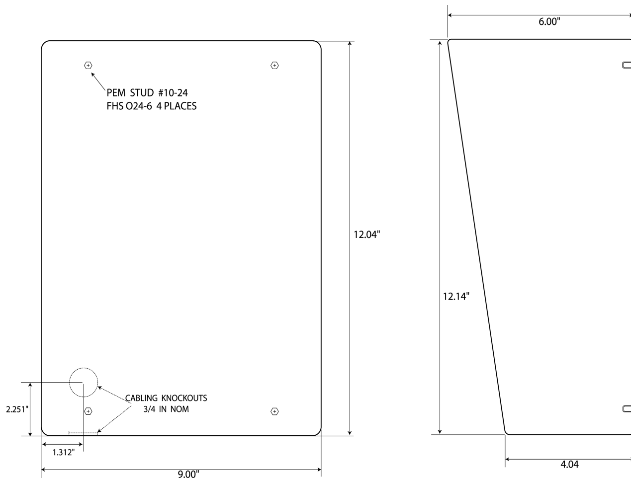
Figure 1: HSE-750 Hooded Mount Dimensions
