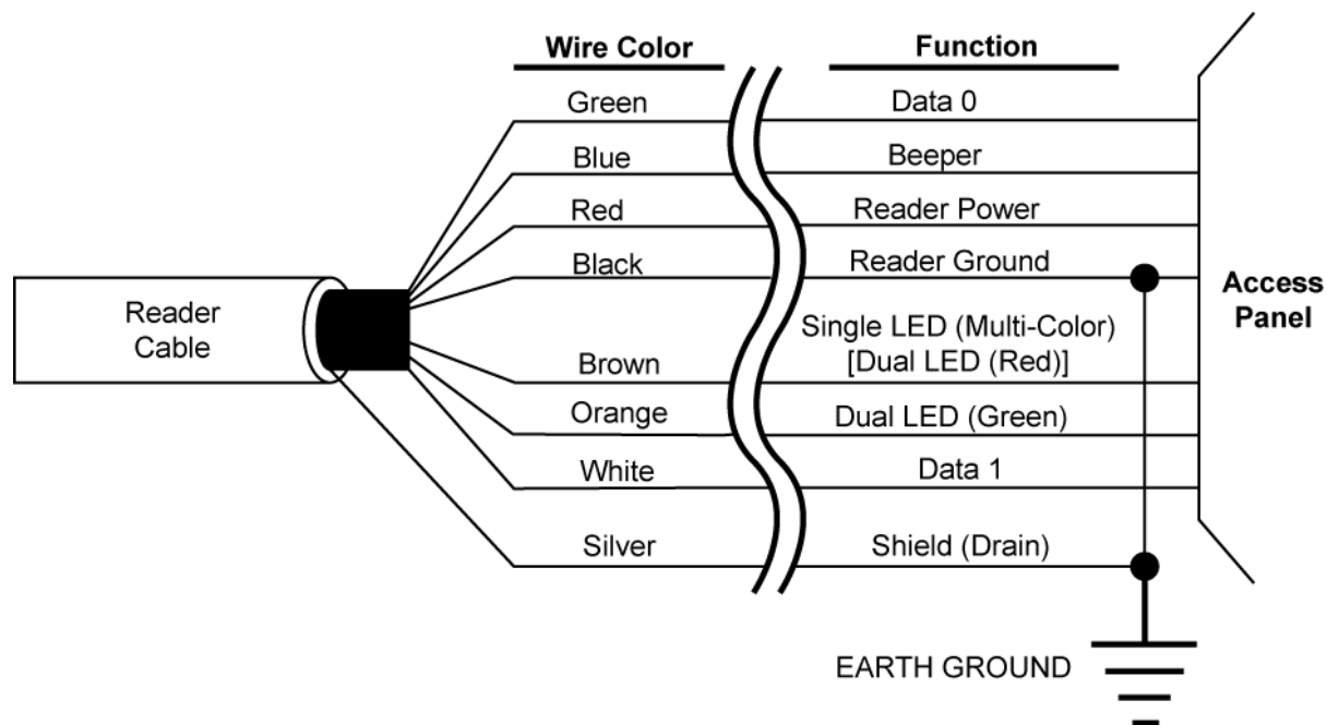
Figure 2: InStar Proximity Reader Wiring Connections
