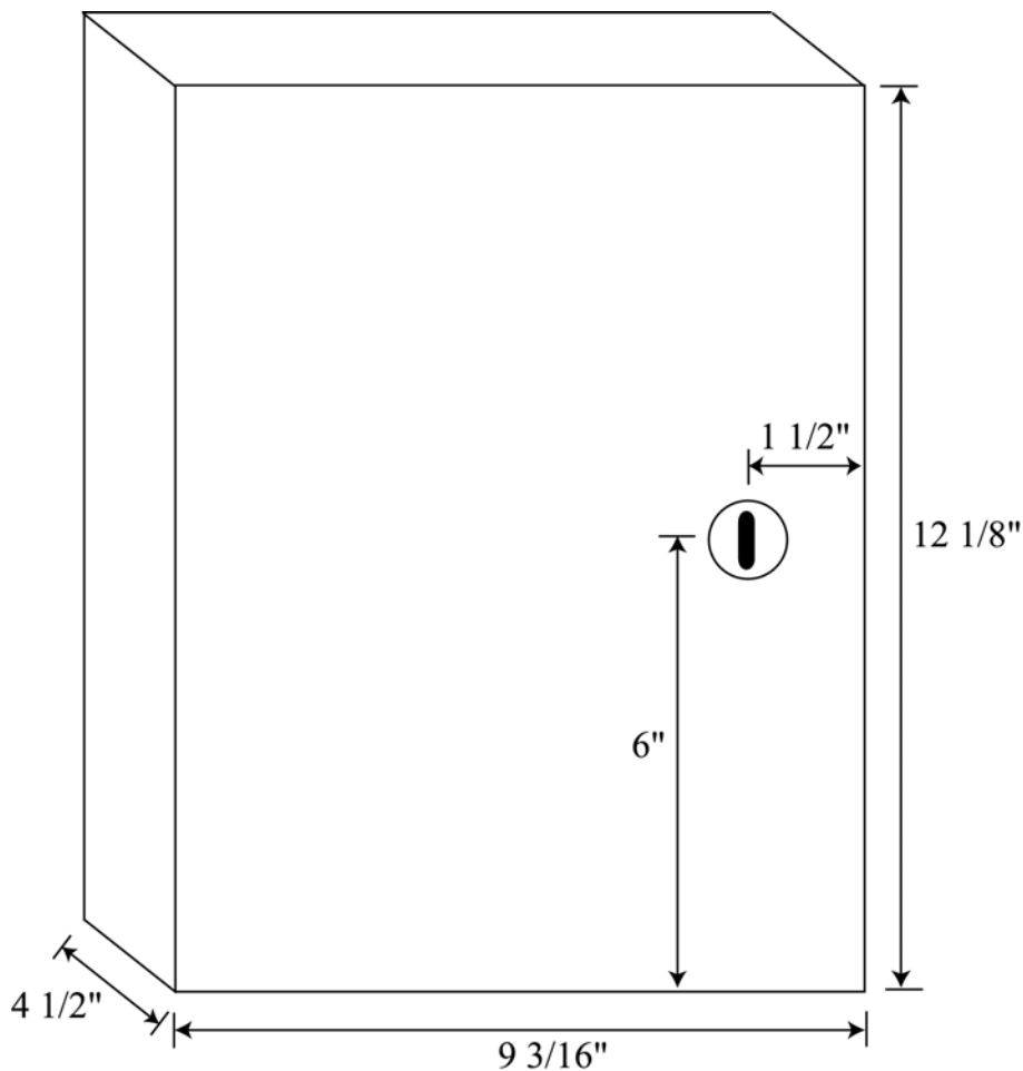
Figure 1: KRE-2 Dimensions
