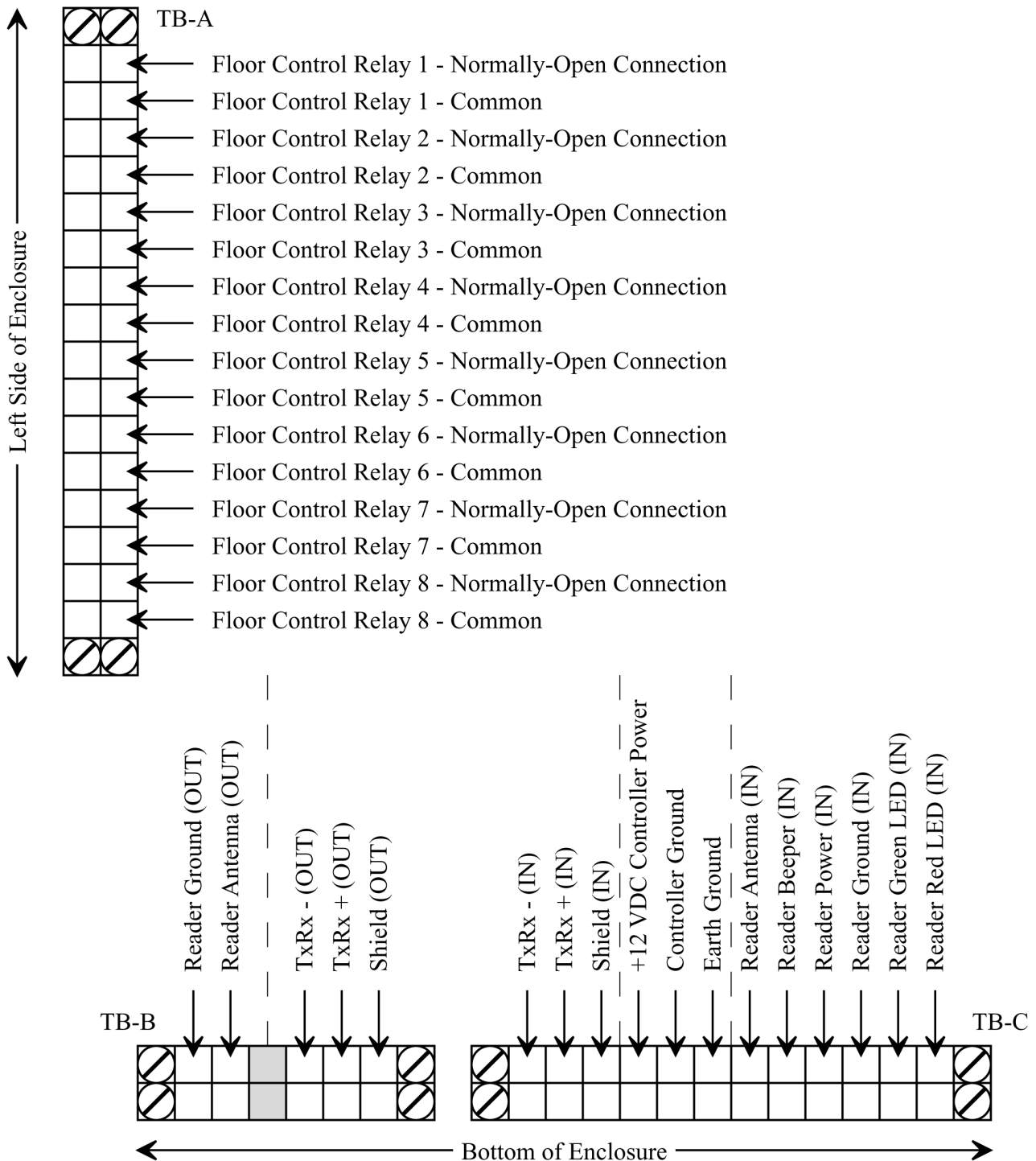
Figure 9: LC-208 Elevator Panel Wiring Connections
