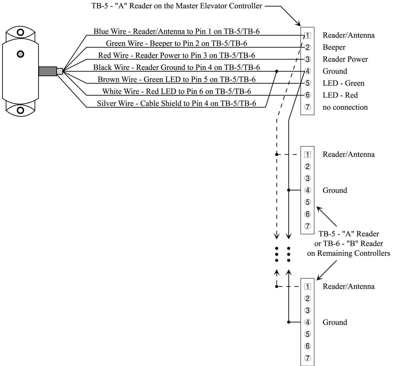
Figure 7: Daisy-Chained Reader Connections
