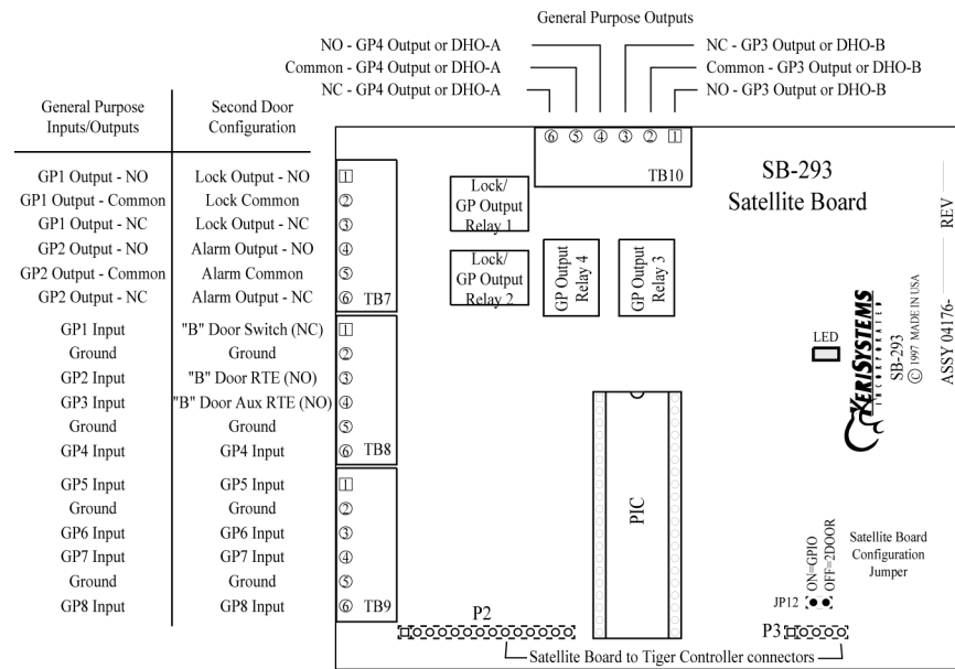
Figure 1: SB-293 Board
