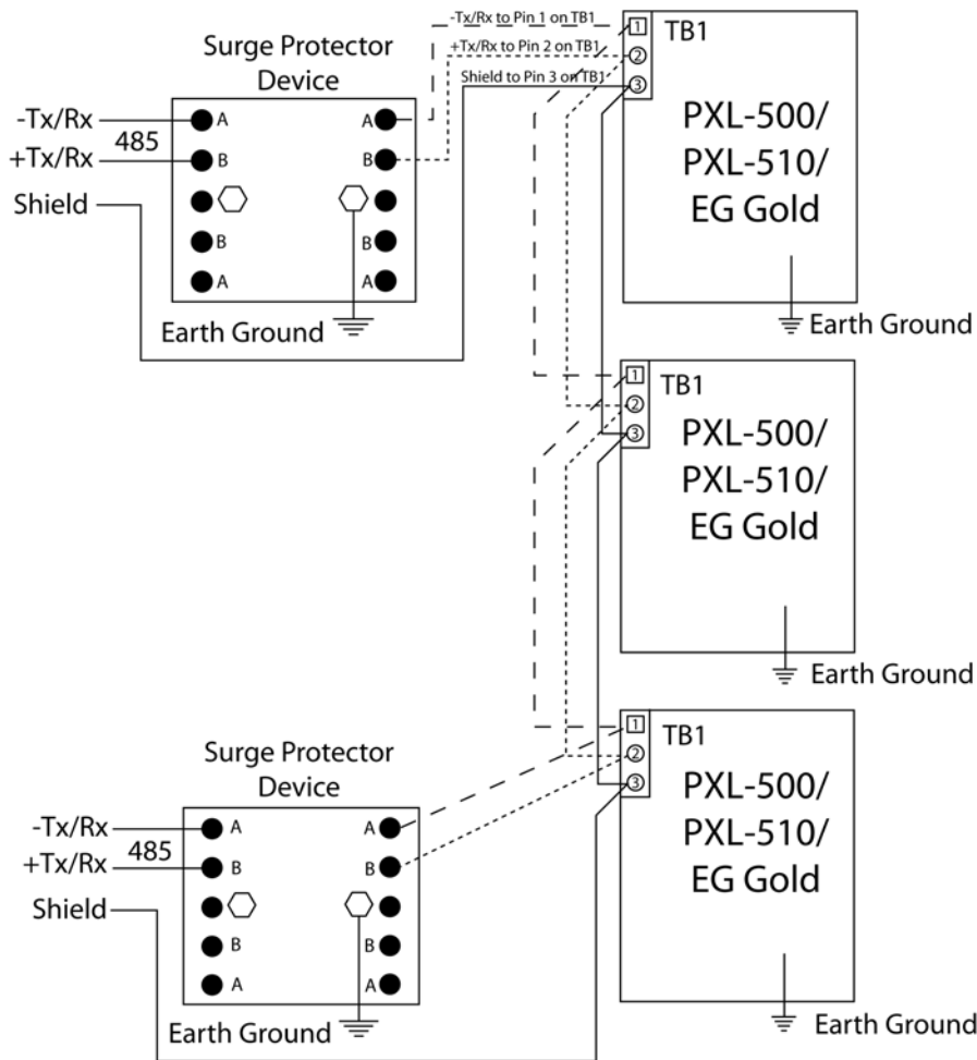
Figure 2: Building or Outside Location Network
