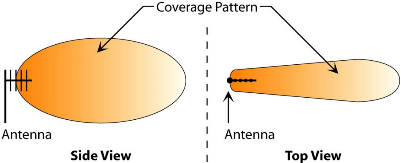
Figure 11: Yagi Antenna Point-to-Point Coverage Pattern
