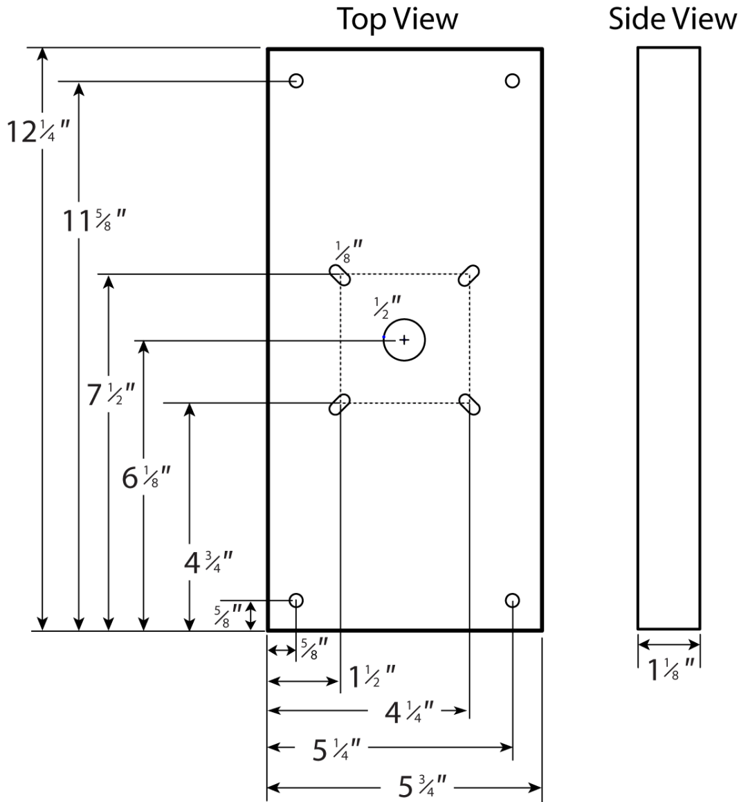
Figure 1: GNA-65 Goose Neck Mount Adapter Dimensions
